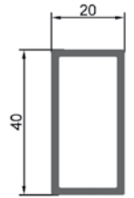
MARCO LATERAL
